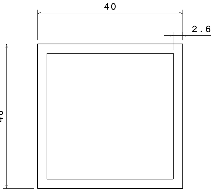
Section Detail of ITEM 1,2, & 3 Scale: 2:1
