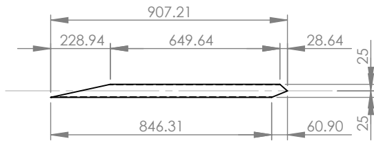
ITEM 6 SHS 50X50X2.0X907.21
