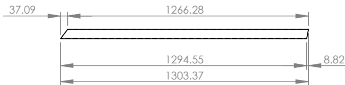
ITEM 11 SHS 50X50X2.0X1303.37
