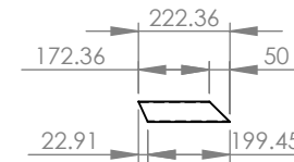
ITEM 12 SHS 50X50X2.0X222.36
