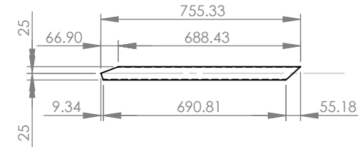
ITEM 8 SHS 50X50X2.0X755.33
