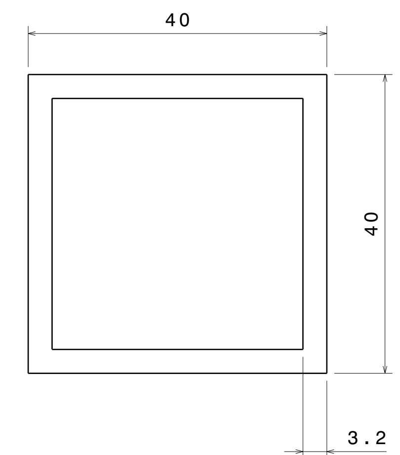
Section Detail of ITEM 1,2,3 & 4 Scale: 2:1
