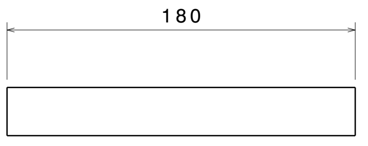
ITEM 6 DETAILS Sq Tube Dog Bed Frame 6
