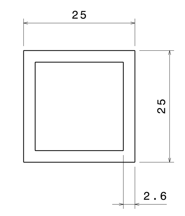
Section Detail of ITEM 5 & 6 Scale: 2:1
