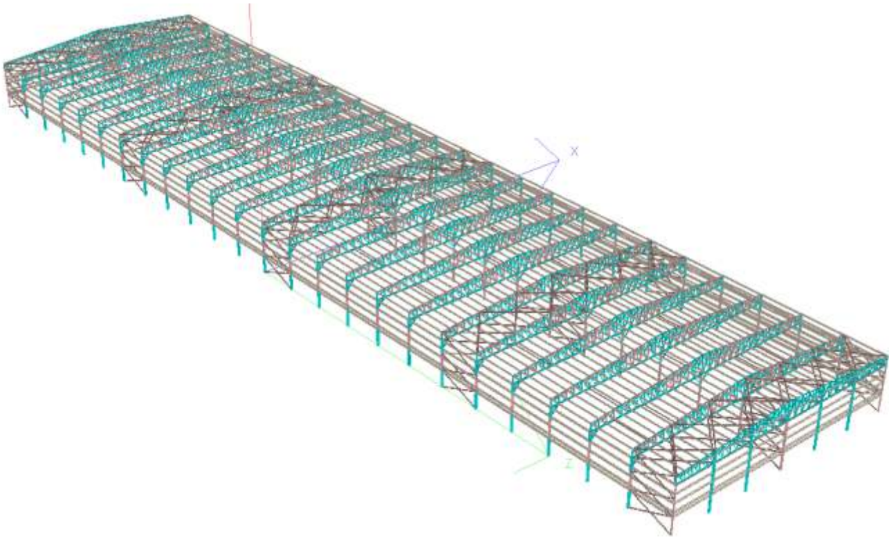
ISOMETRIC VIEW
