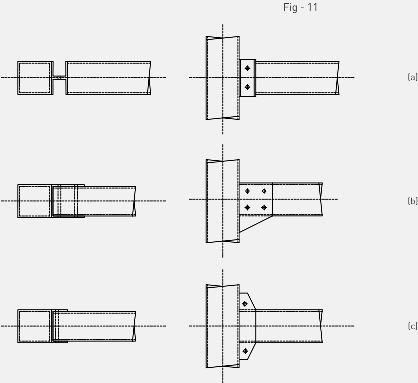
Typical connection of an RHS beam to an RHS column a,b&c
