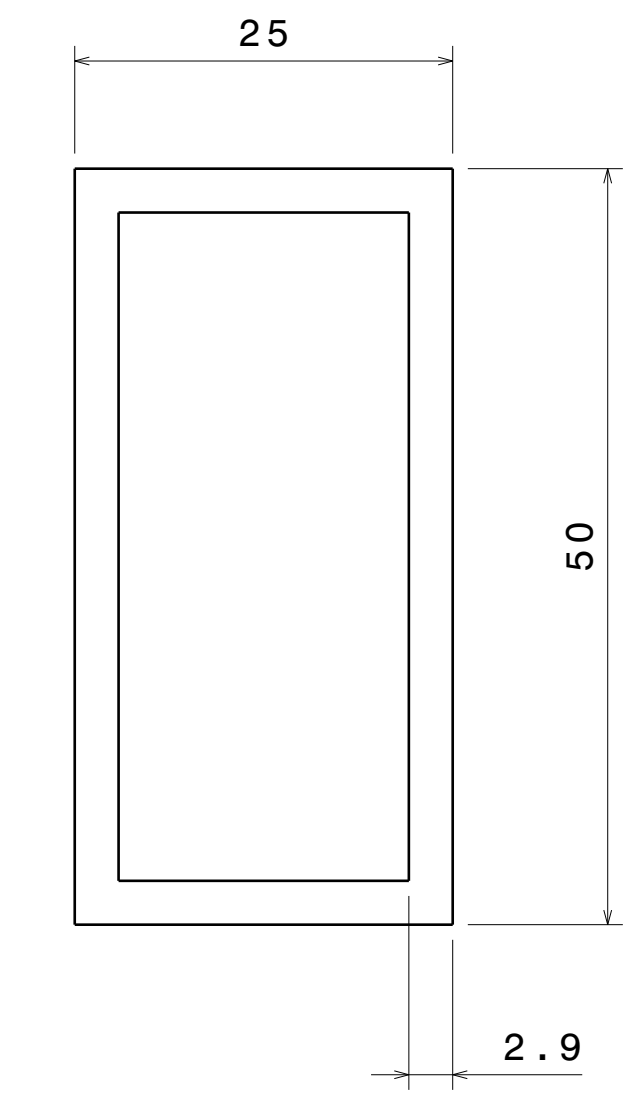
Section Detail of ITEM 3 Scale: 2:1
