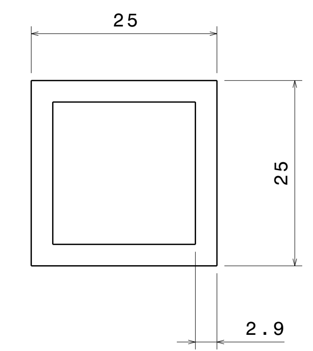
Section Detail of ITEM 1, 2, 4 & 5 Scale: 2:1
