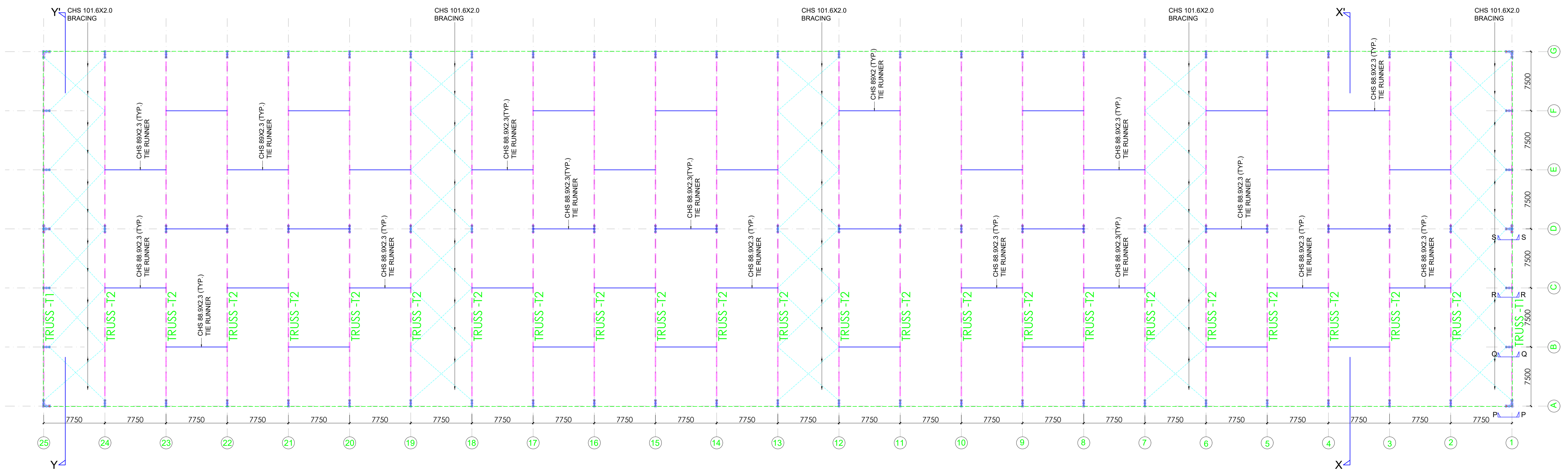
BOTTOM CHORD PLAN
