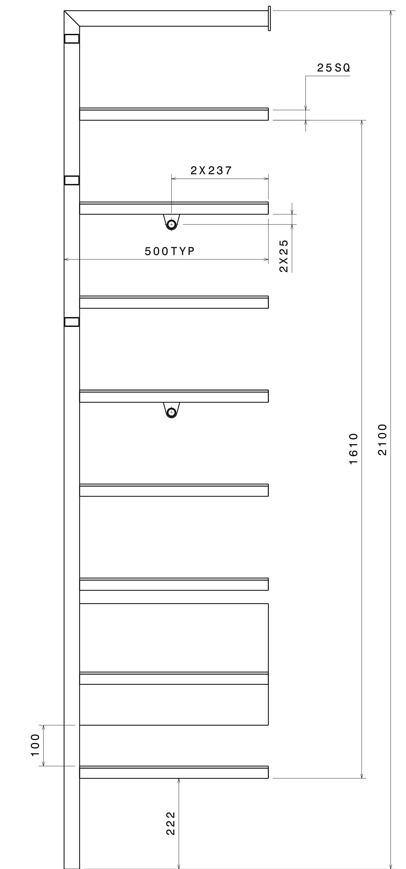
Right view
