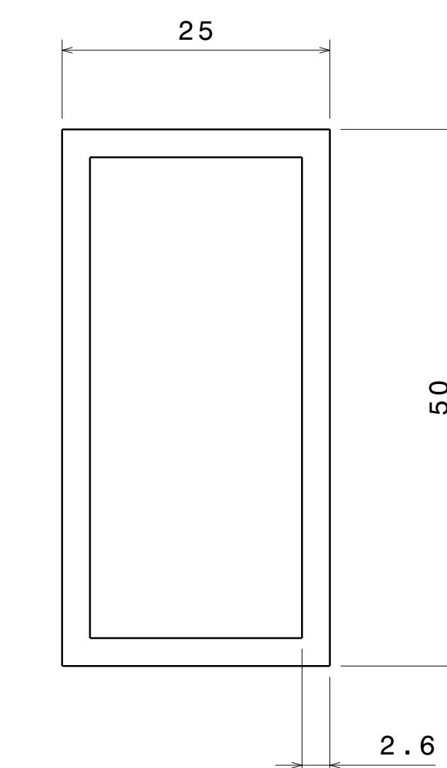
Section Detail of ITEM 5 & 6 Scale: 2:1
