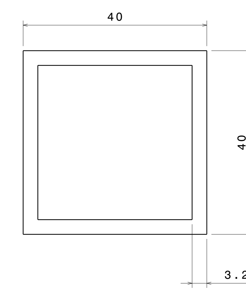
Section Detail of ITEM 1 & 2 Scale: 2:1
