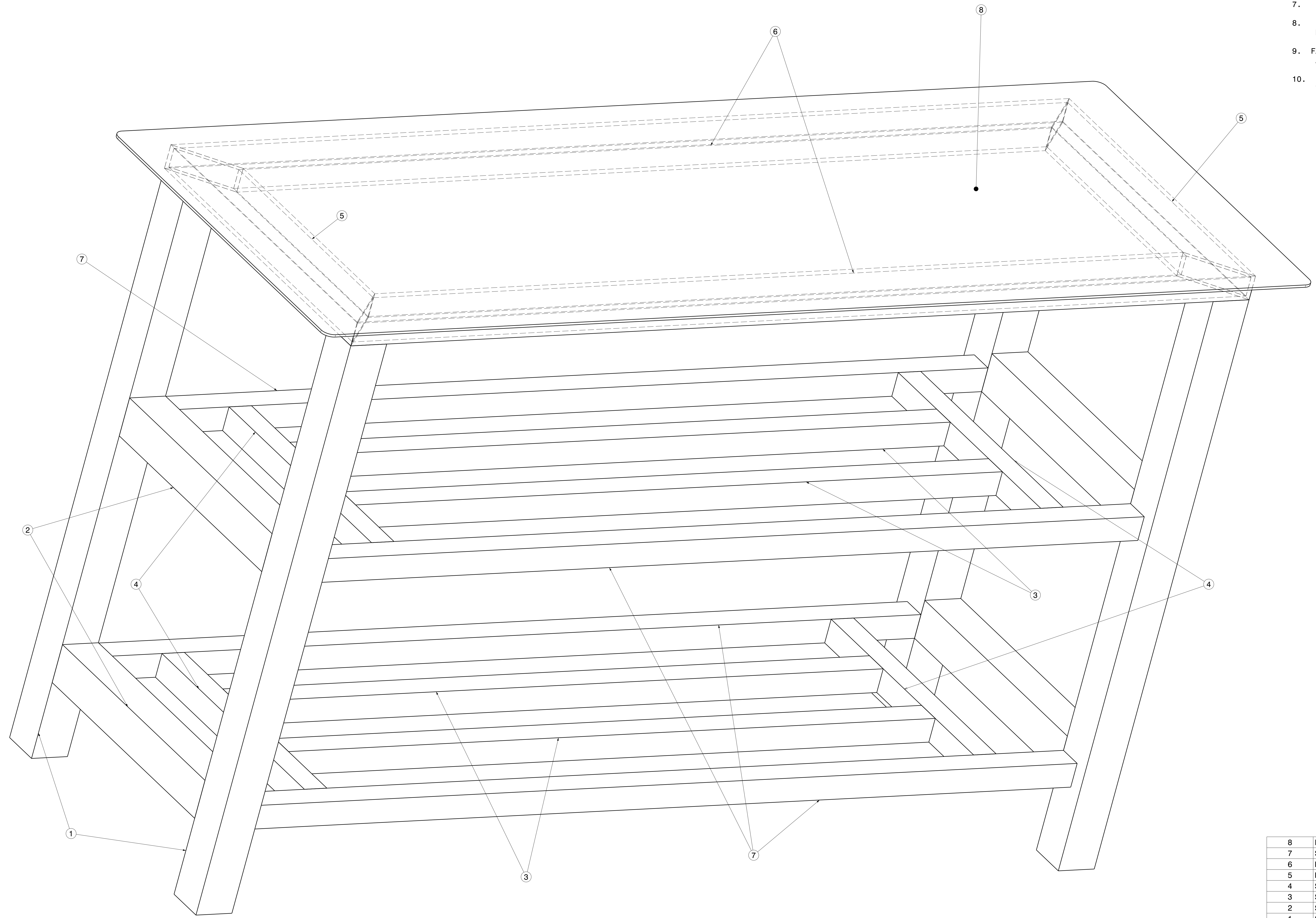
Isometric view Scale: 7:10
