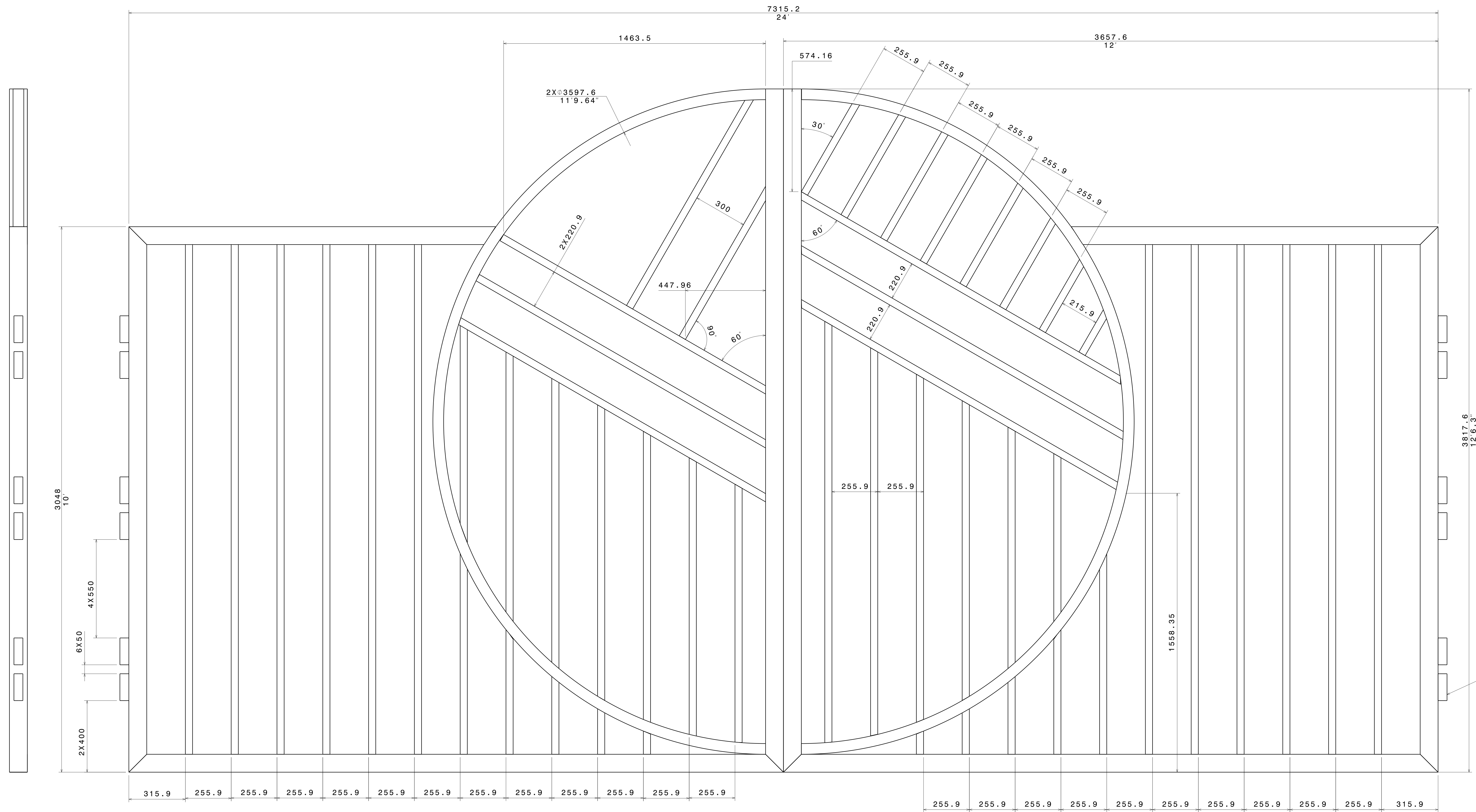
FRONT VIEW
