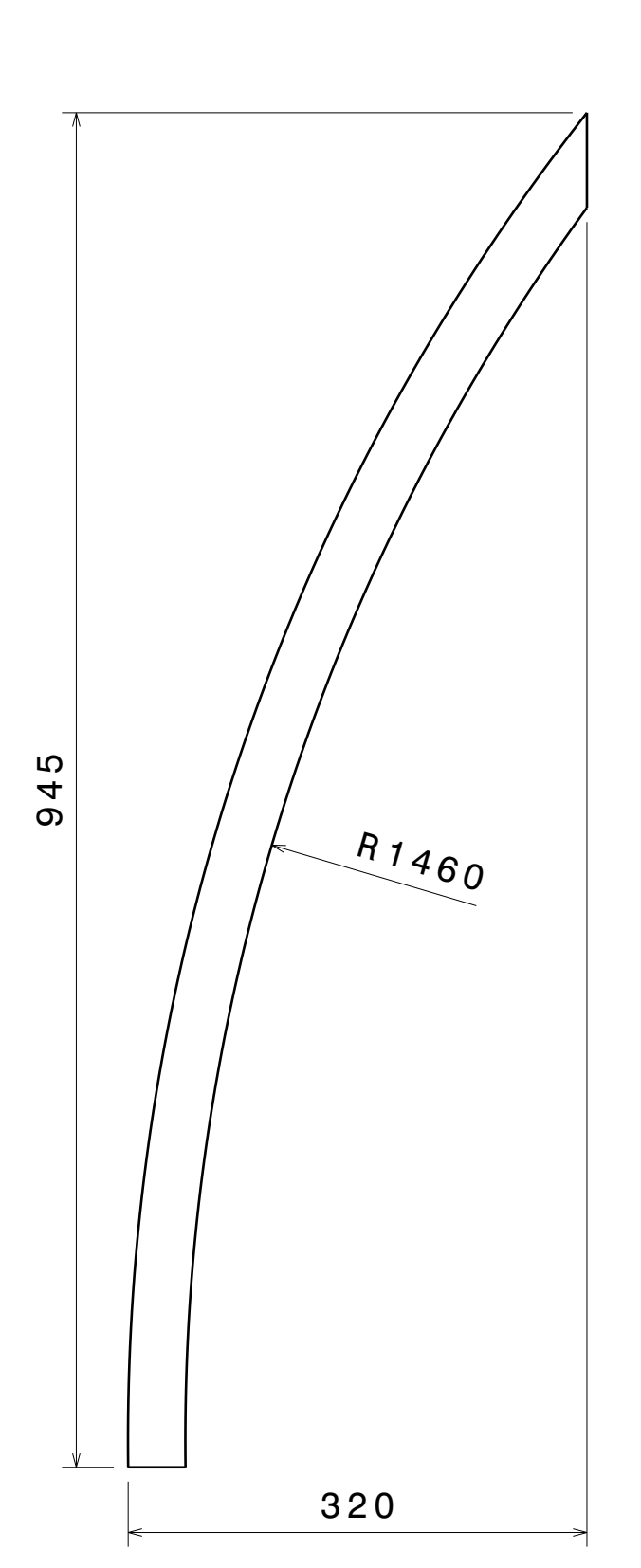
ITEM 6 DETAILS Sq_tube 33.1 Frame 6
