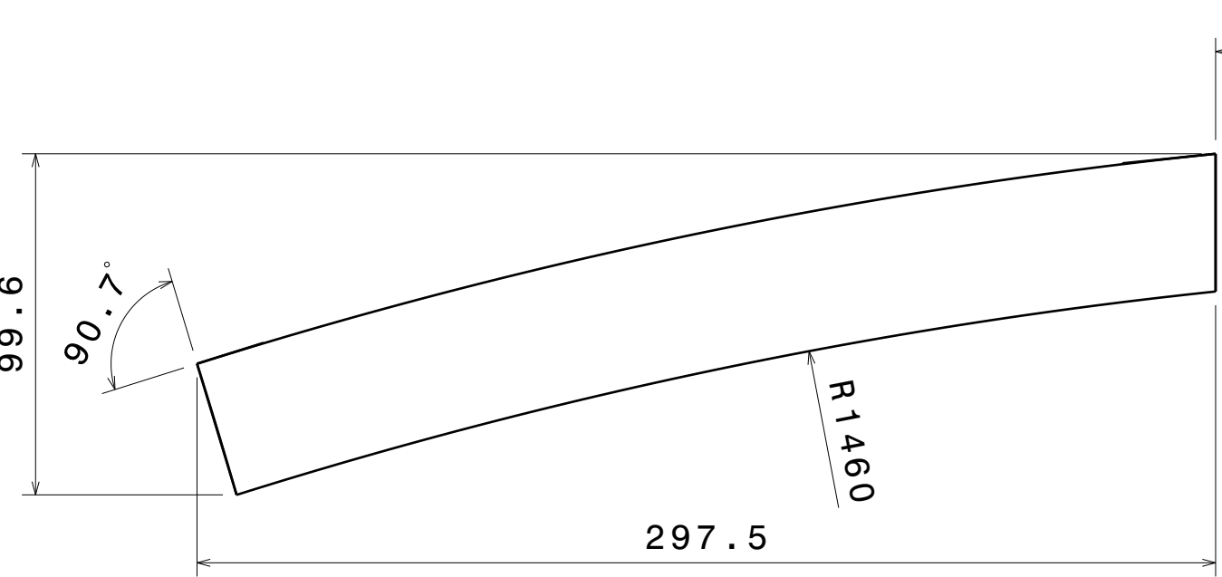
ITEM 20 DETAILS Sq_tube 33.1 Frame 20
