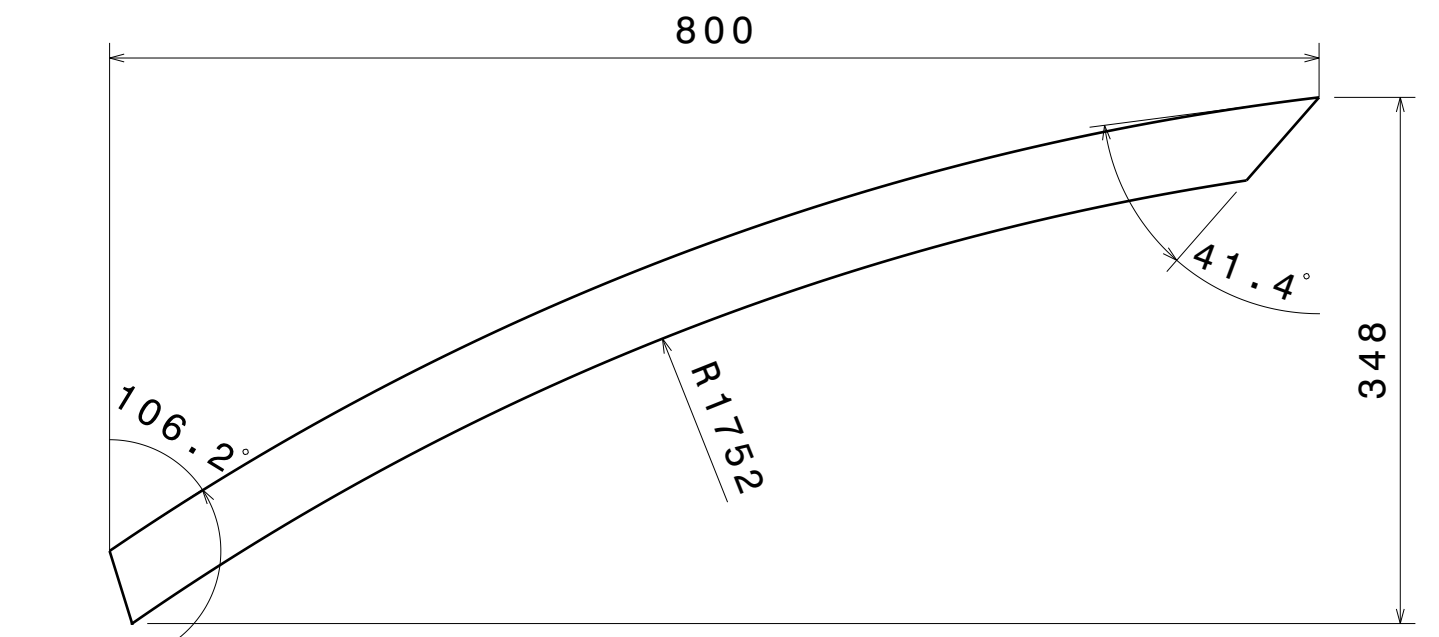
ITEM 3 DETAILS rect_tube 33.1 Frame 3
