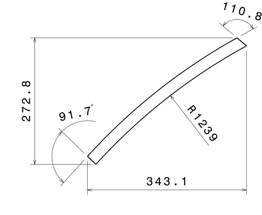
ITEM 29 DETAILS Sq_tube 33.1 Frame 29
