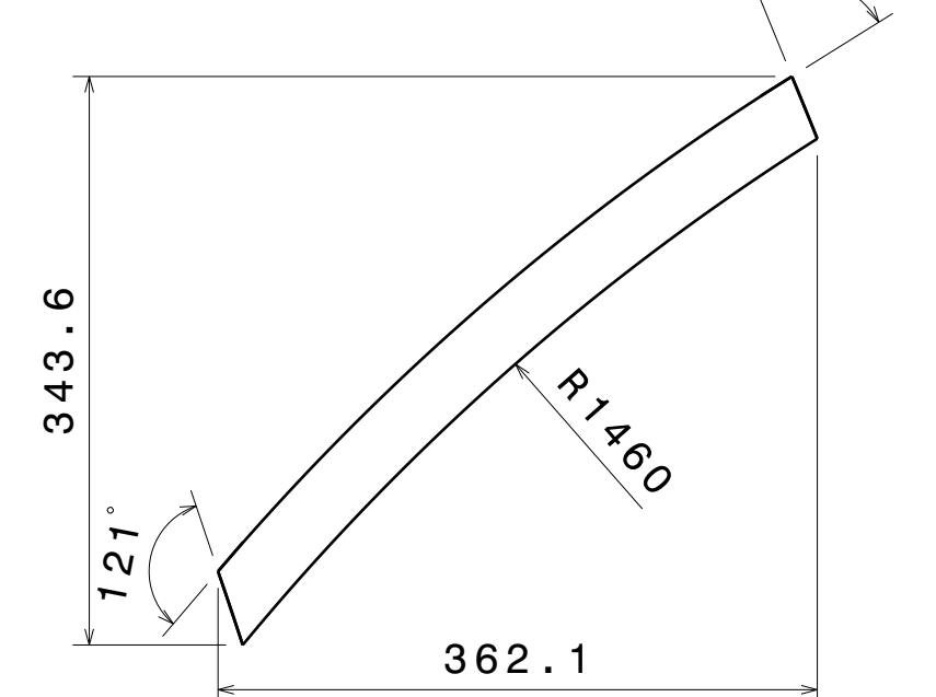
ITEM 11 DETAILS Sq_tube 33.1 Frame 11
