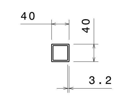
Section Detail of ITEM 6,7,8,9,10,11,12,13, 14,15,16,17,18,19, 20,21 & 22 Scale: 1:5
