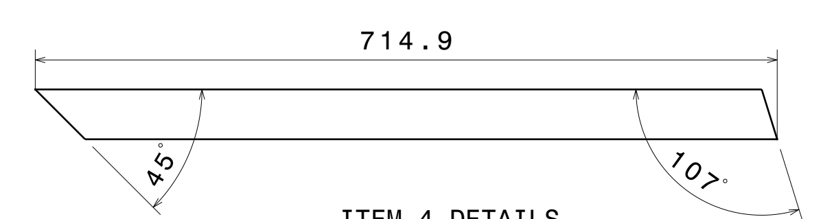
ITEM 4 DETAILS rect_tube 33.1 Frame 4
