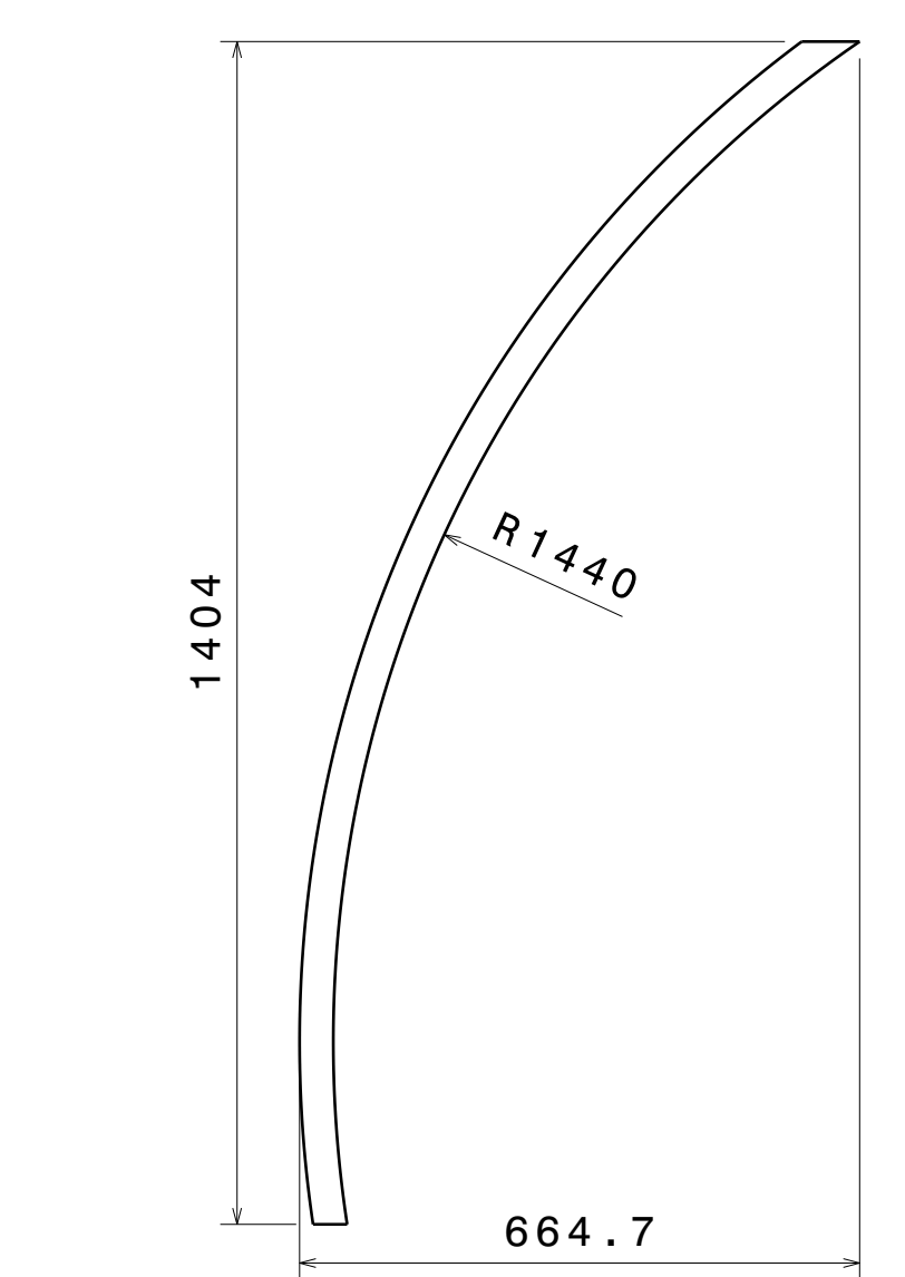
ITEM 8 DETAILS Sq_tube 33.1 Frame 8
