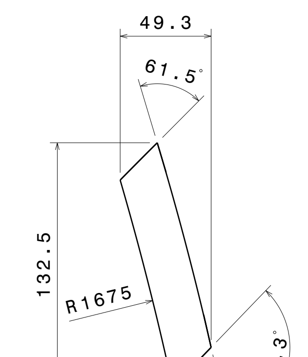
ITEM 33 DETAILS Sq_tube 33.1 Frame 33
