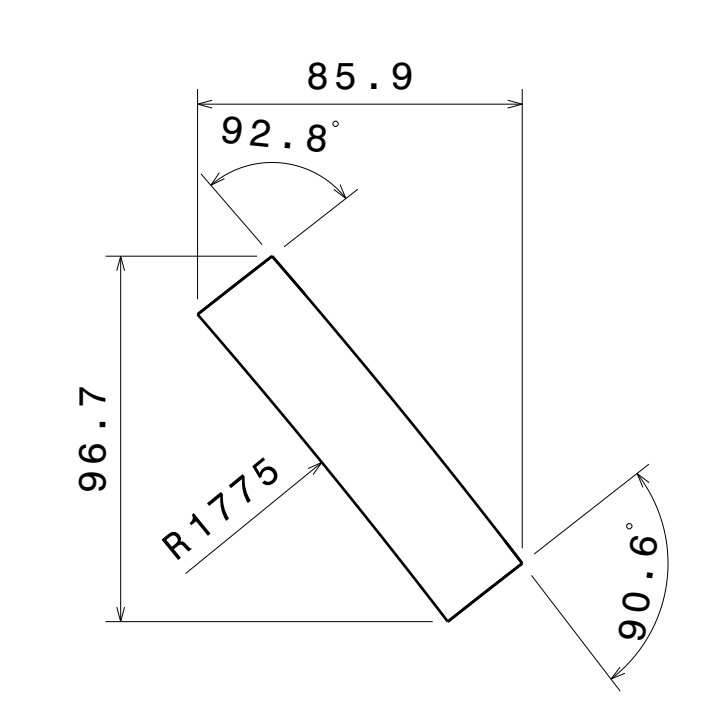
ITEM 36 DETAILS Sq_tube 33.1 Frame 36
