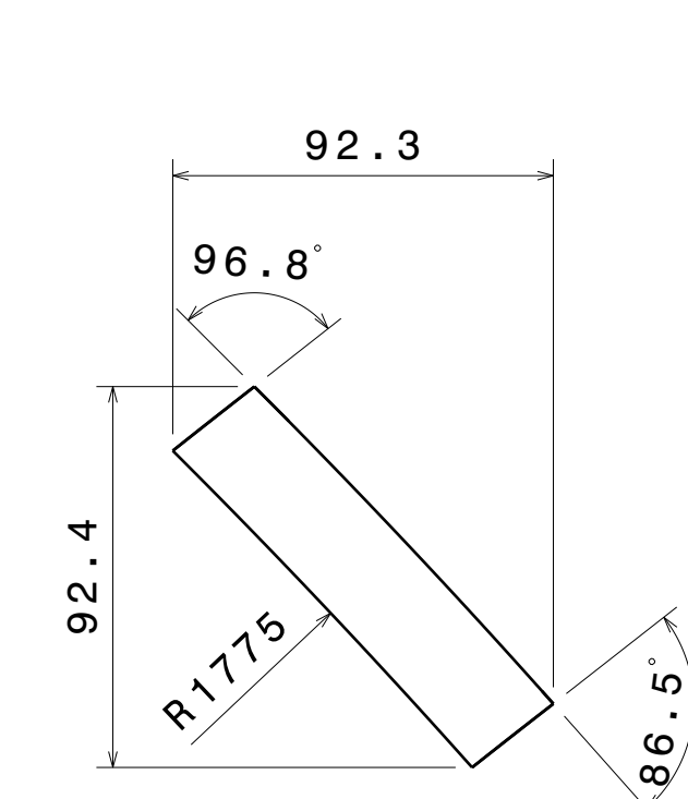
ITEM 37 DETAILS Sq_tube 33.1 Frame 37
