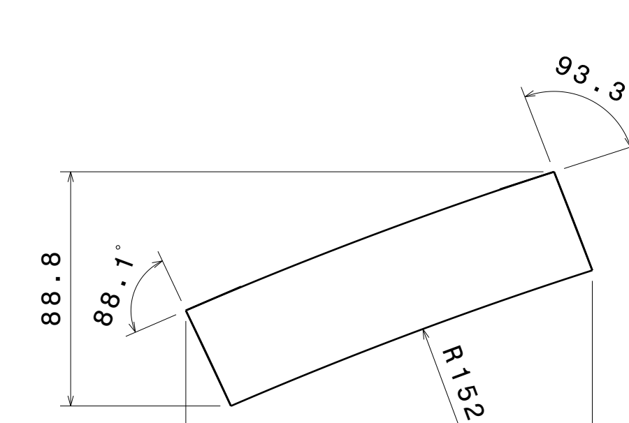
ITEM 18 DETAILS Sq_tube 33.1 Frame 18
