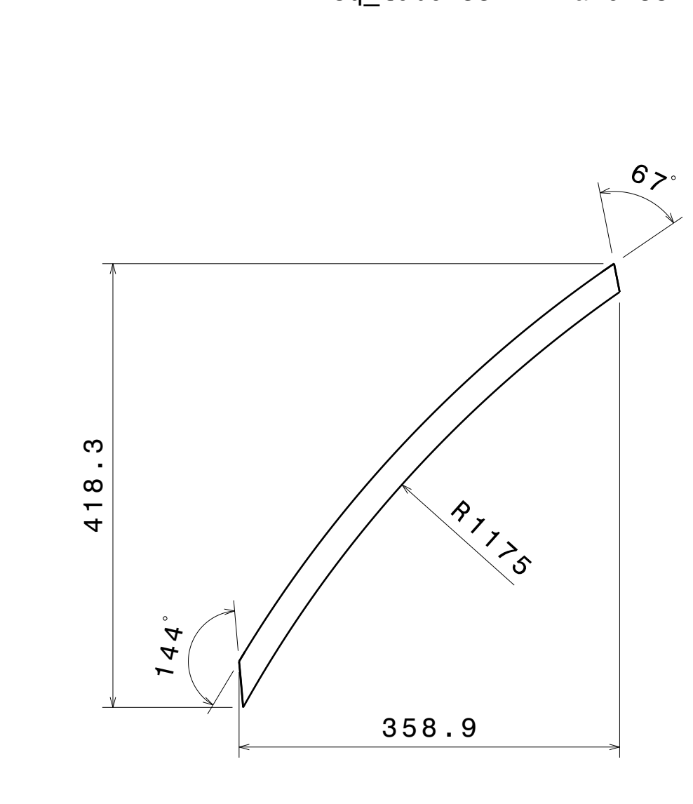
ITEM 25 DETAILS Sq_tube 33.1 Frame 25
