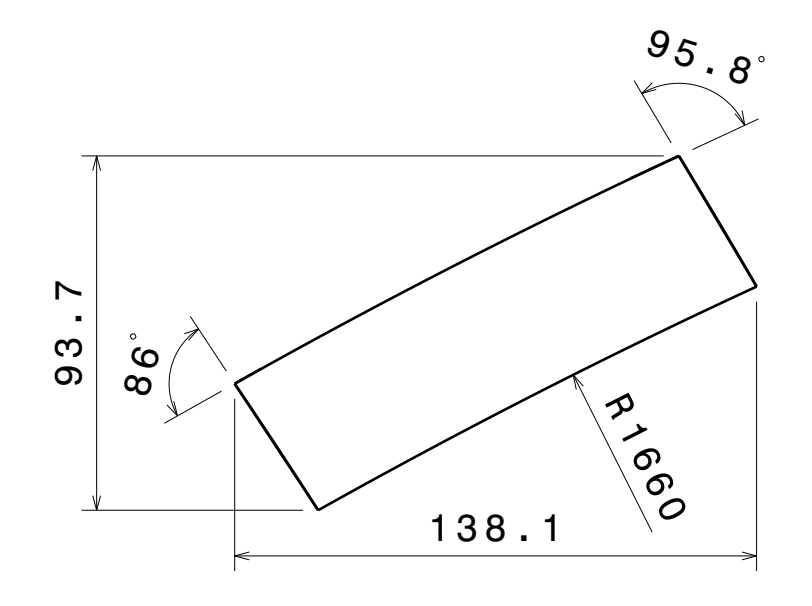
ITEM 16 DETAILS Sq_tube 33.1 Frame 16
