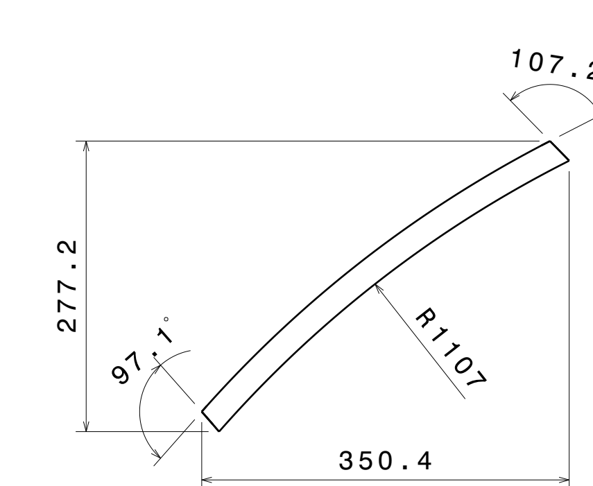
ITEM 28 DETAILS Sq_tube 33.1 Frame 28
