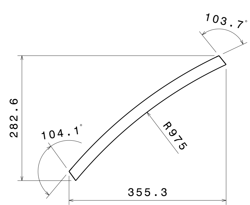
ITEM 27 DETAILS Sq_tube 33.1 Frame 27
