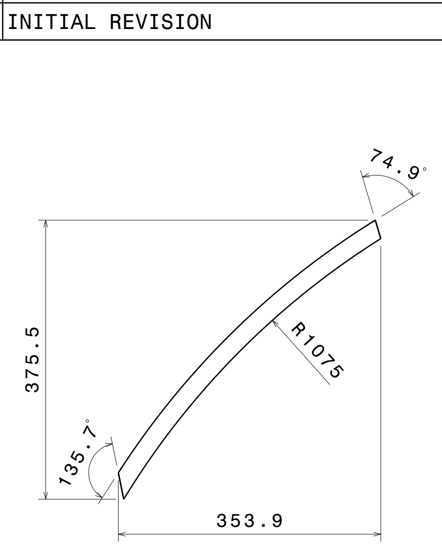
ITEM 26 DETAILS Sq_tube 33.1 Frame 26
