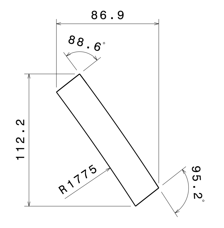
ITEM 35 DETAILS Sq_tube 33.1 Frame 35
