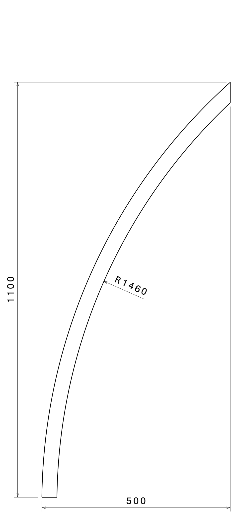
ITEM 7 DETAILS Sq_tube 33.1 Frame 7
