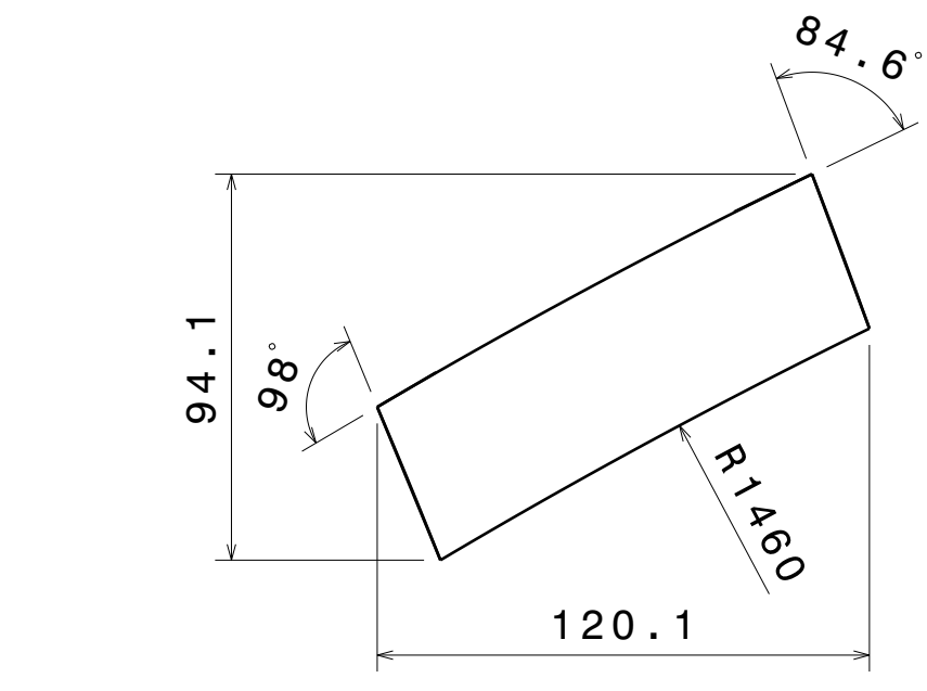
ITEM 14 DETAILS Sq_tube 33.1 Frame 14
