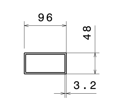
Section Detail of ITEM 1,2,3 & 4 Scale: 1:5
