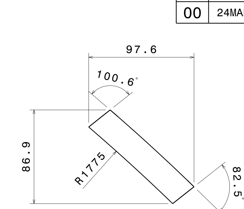
ITEM 38 DETAILS Sq_tube 33.1 Frame 38
