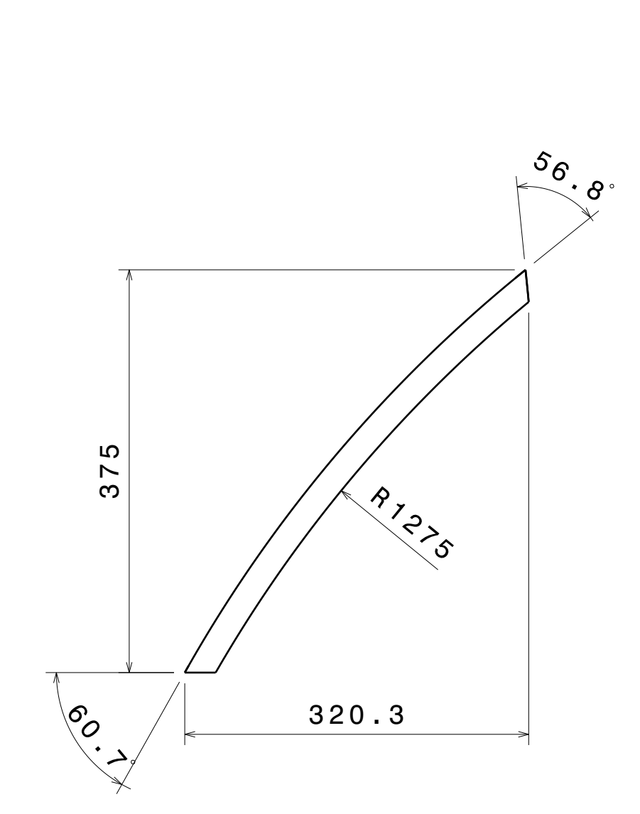
ITEM 24 DETAILS Sq_tube 33.1 Frame 24
