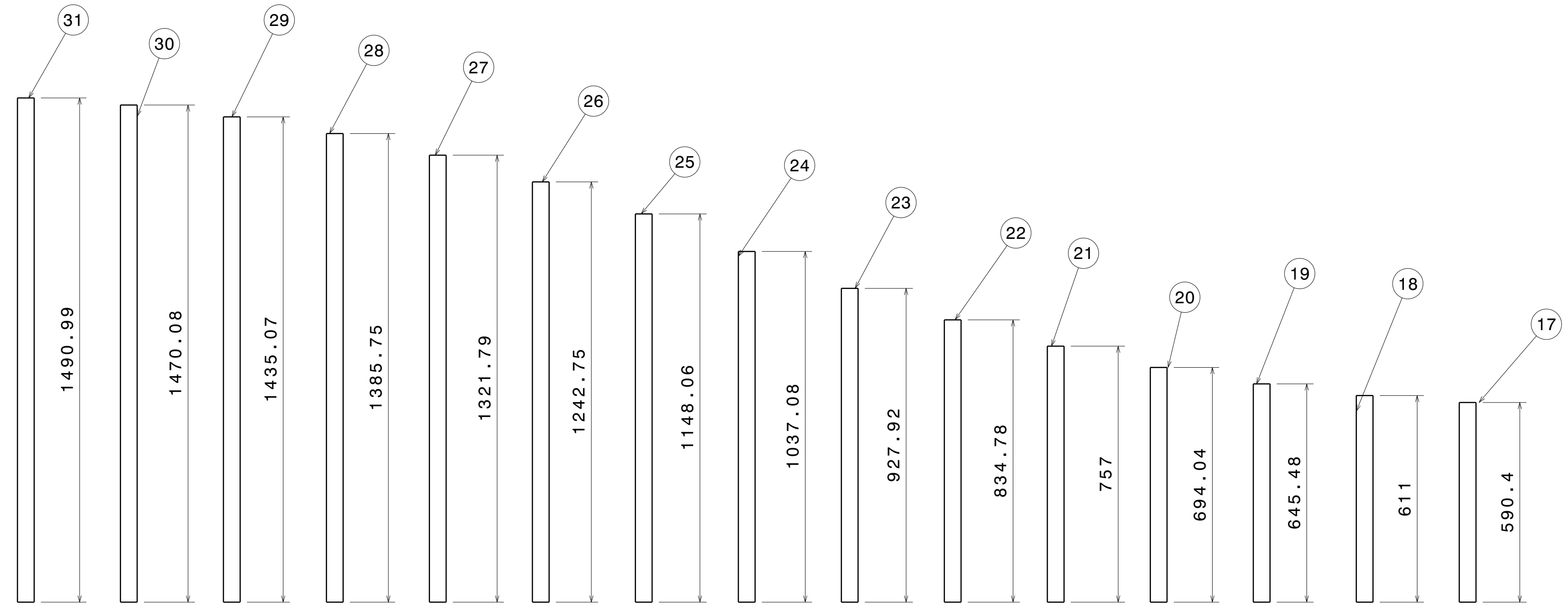
ITEM 6 TO ITEM 16 ARE OF SAME SQUARE CROSS SECTION: 49.5 SQ X 2.6 THK
