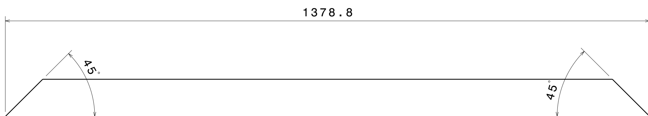
ITEM 2 DETAILS Sq tube 35.1 Frame 2
