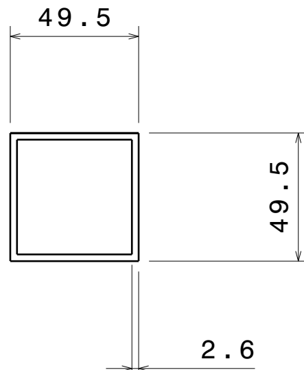
Section Detail of ITEM 5,6,7,8,9,10,11 & 12 Scale: 1:2
