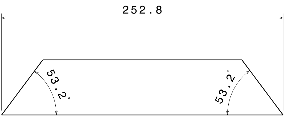
ITEM 12 DETAILS Sq tube 35.1 Frame 11
