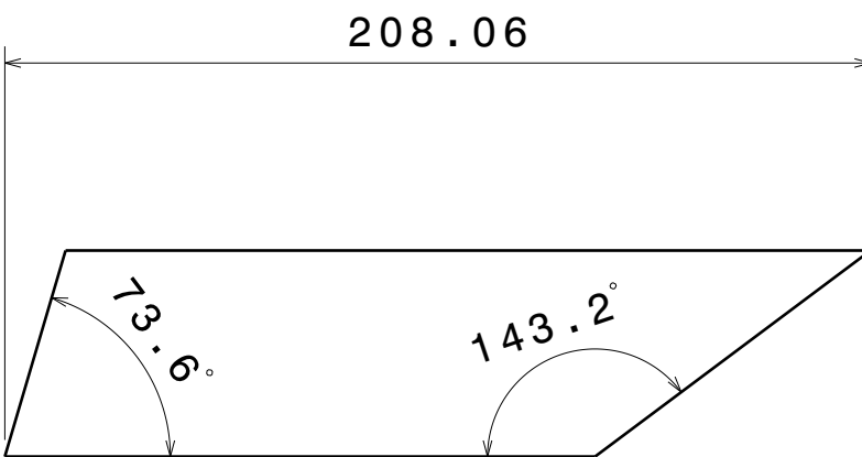
ITEM 9 DETAILS Sq tube 35.1 Frame 8
