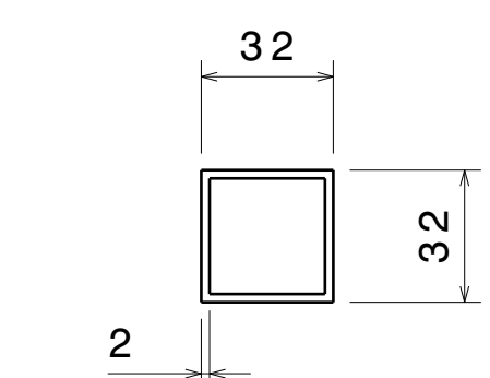
Section Detail of ITEM 4,8,9,10,11,12,13,14,15,16,17 & 18 Scale: 1:2
